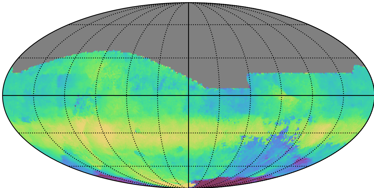
baseline_v3.2_10yrs All sky r band: Median HA
