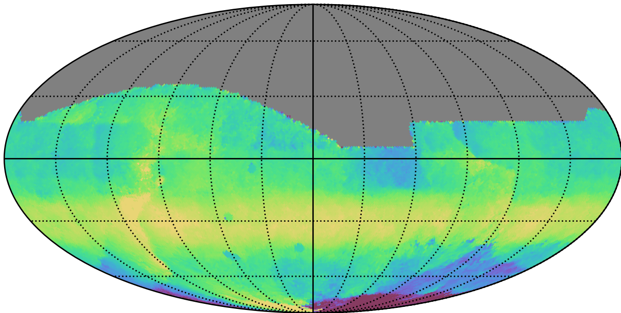
baseline_v3.2_10yrs All sky i band: Median HA
