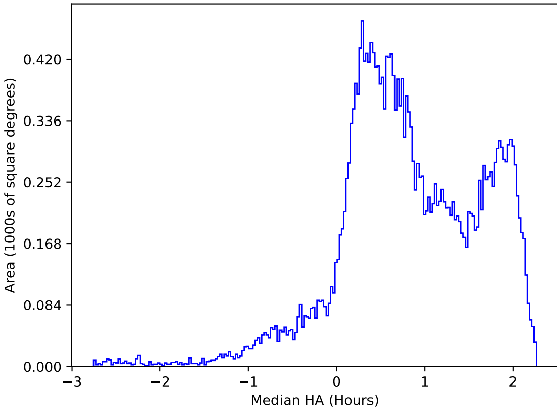
baseline_v3.2_10yrs All sky i band: Median HA
