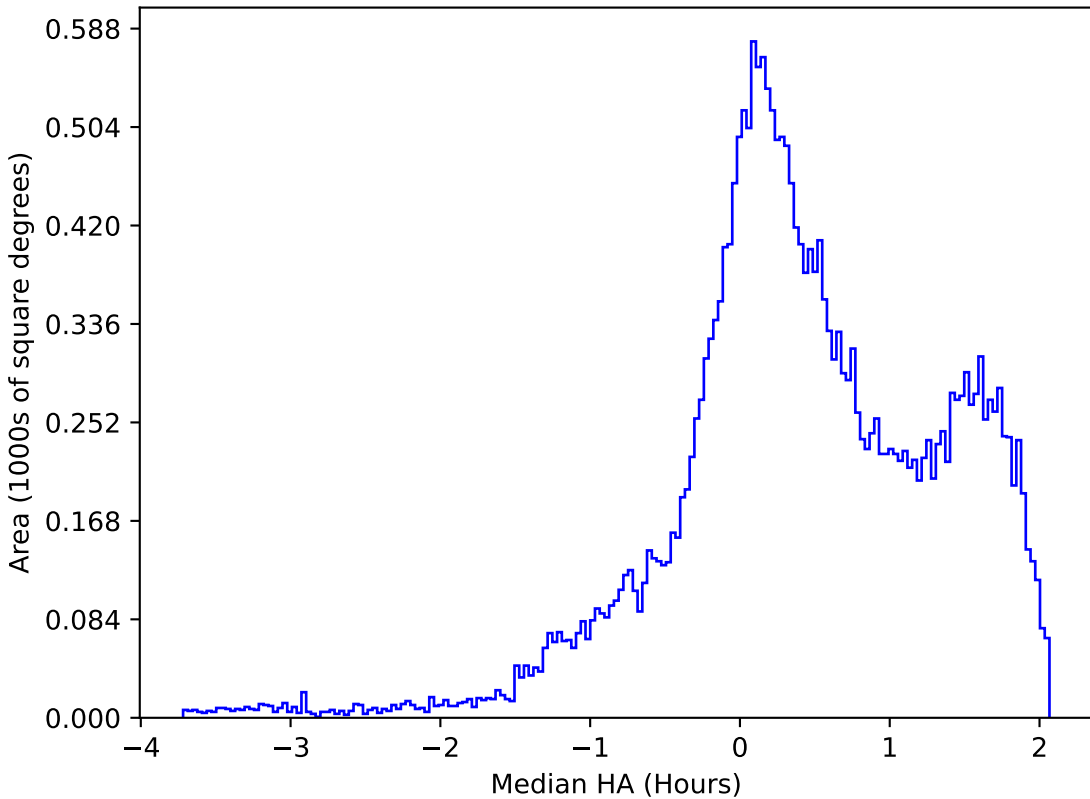
baseline_v3.2_10yrs All sky g band: Median HA
