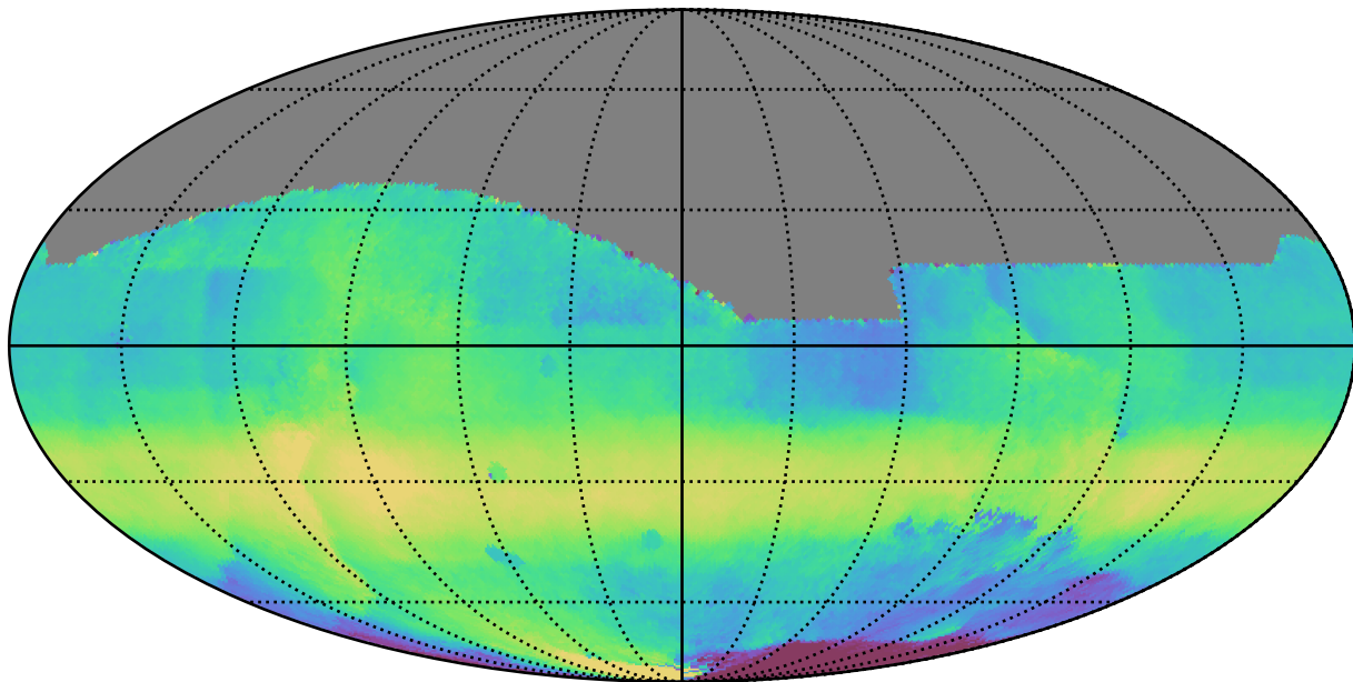
baseline_v3.2_10yrs All sky all bands: Median HA
