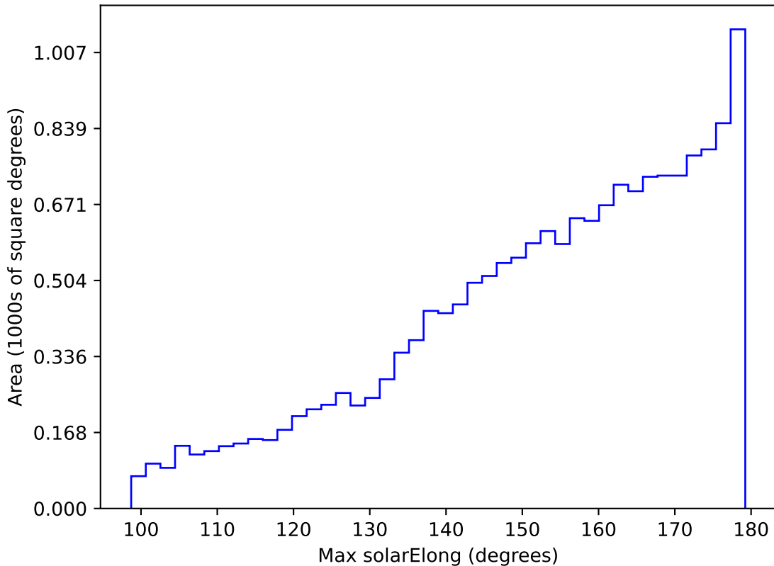
baseline_v3.2_10yrs WFD z band: Max solarElong
