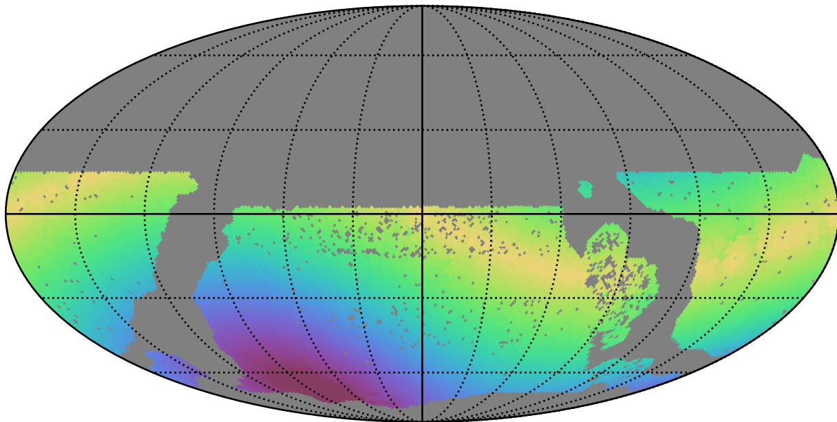
baseline_v3.2_10yrs WFD u band: Max solarElong
