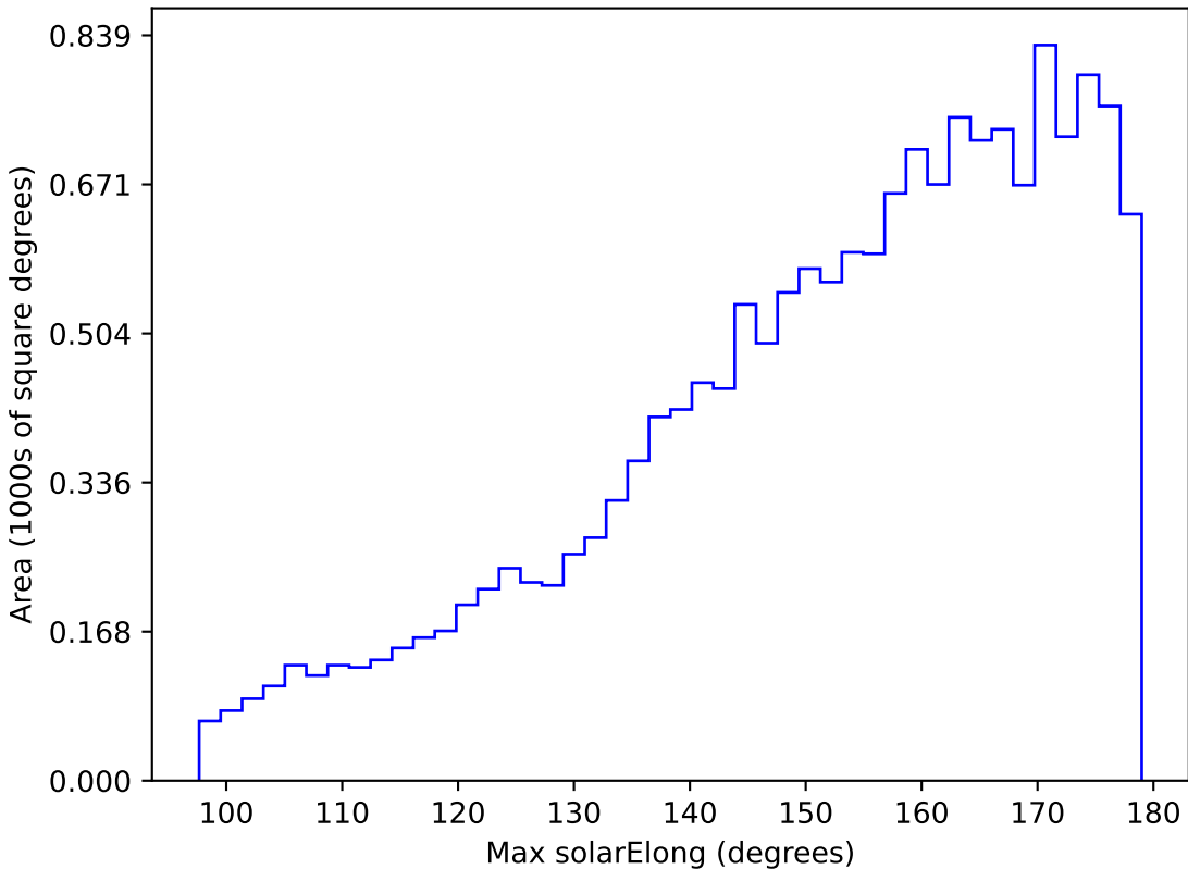
baseline_v3.2_10yrs WFD u band: Max solarElong
