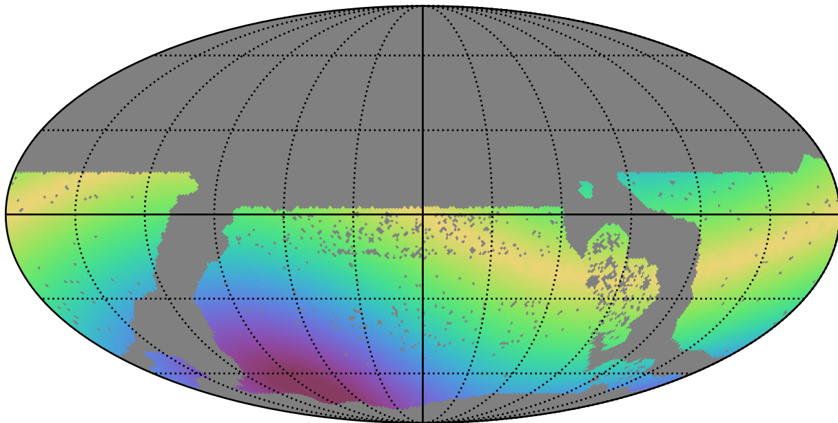
baseline_v3.2_10yrs WFD r band: Max solarElong
