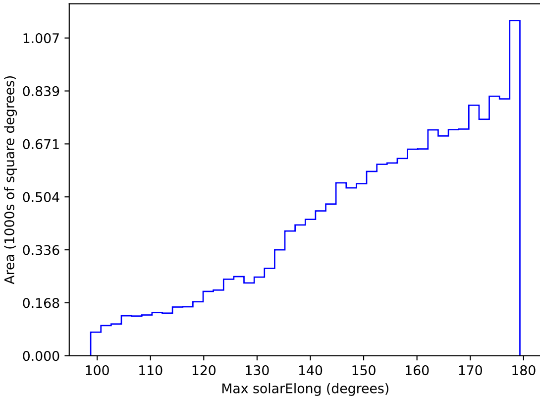
baseline_v3.2_10yrs WFD r band: Max solarElong
