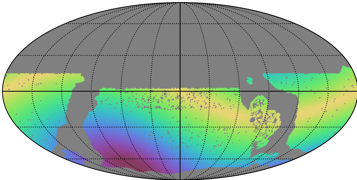
baseline_v3.2_10yrs WFD i band: Max solarElong
