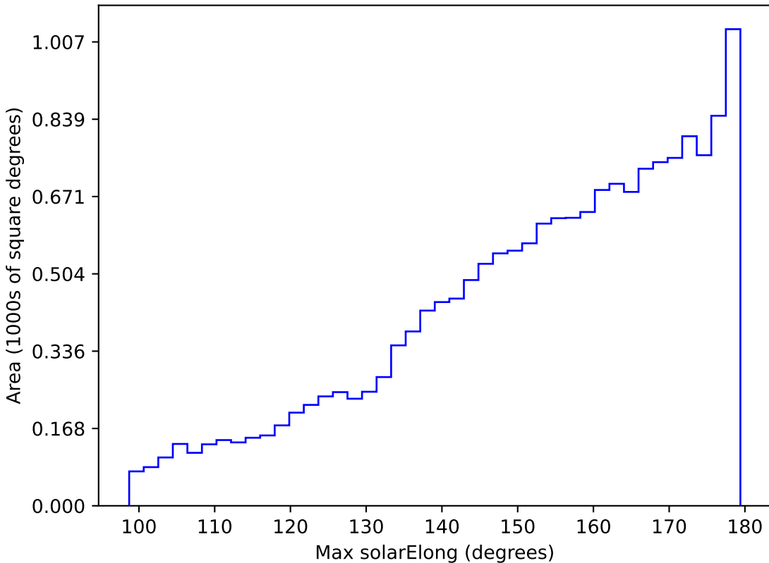
baseline_v3.2_10yrs WFD i band: Max solarElong
