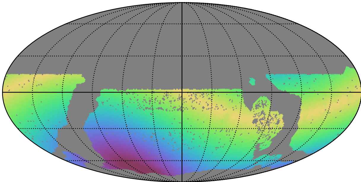
baseline_v3.2_10yrs WFD g band: Max solarElong
