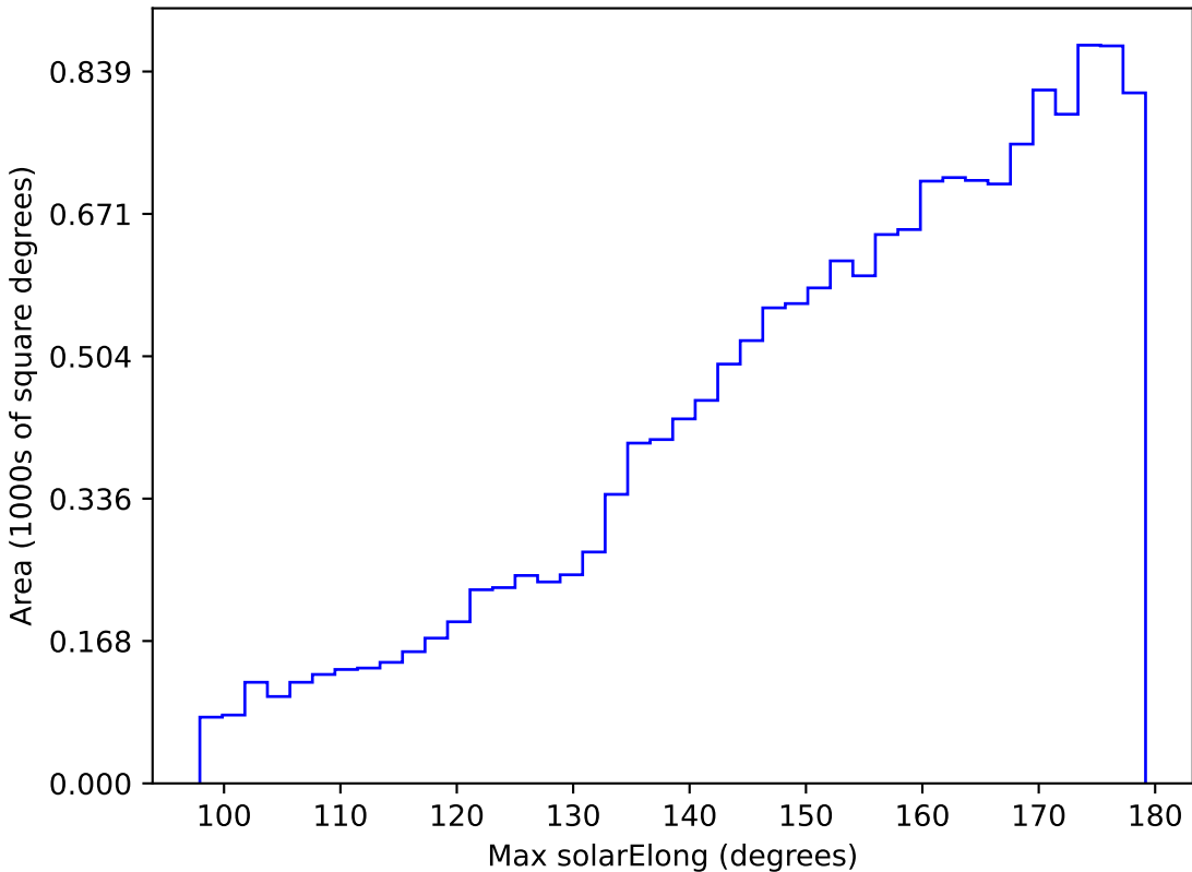
baseline_v3.2_10yrs WFD g band: Max solarElong
