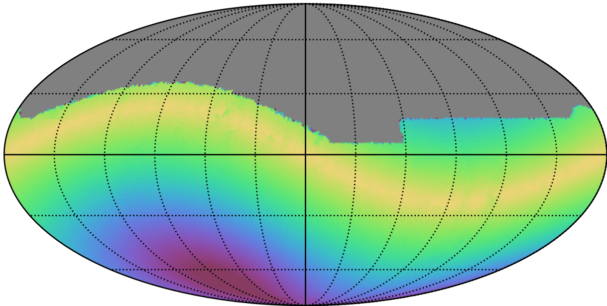
baseline_v3.2_10yrs All sky z band: Max solarElong
