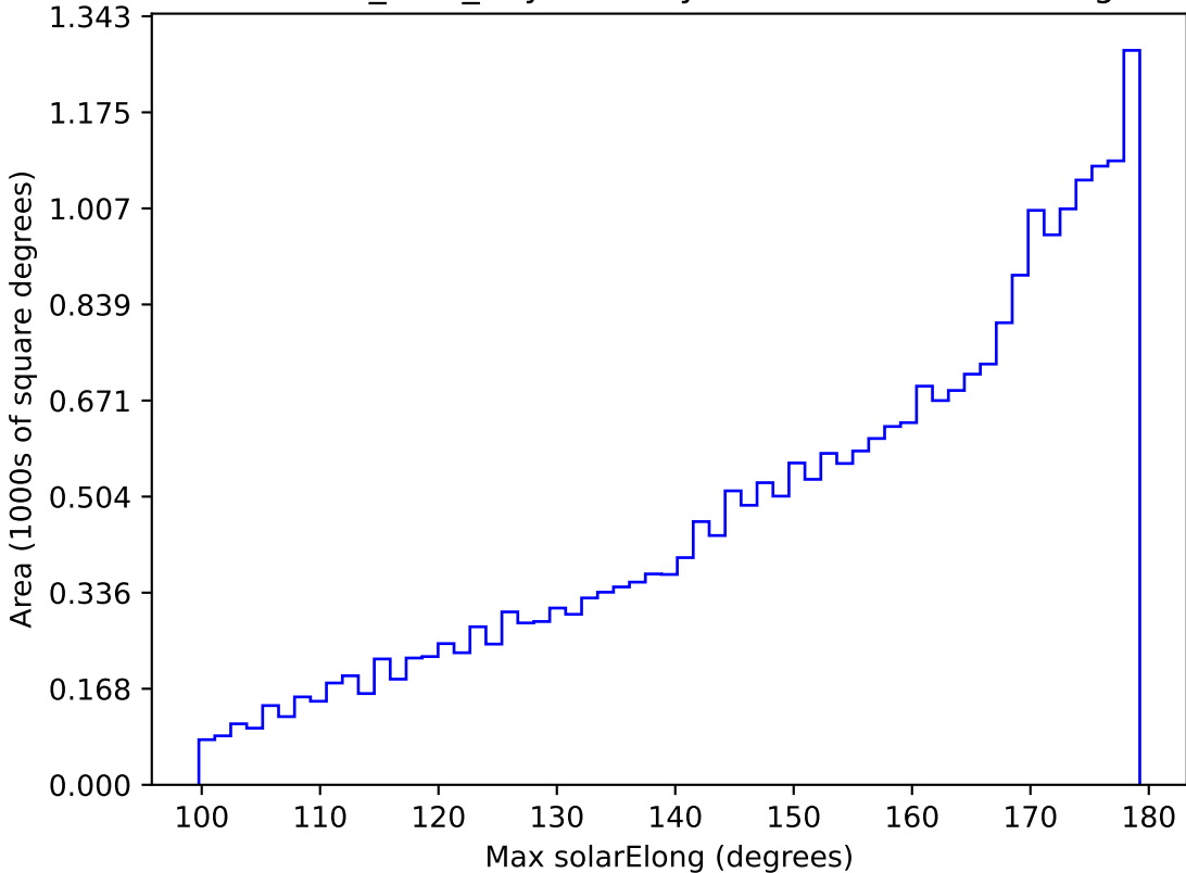
baseline_v3.2_10yrs All sky z band: Max solarElong
