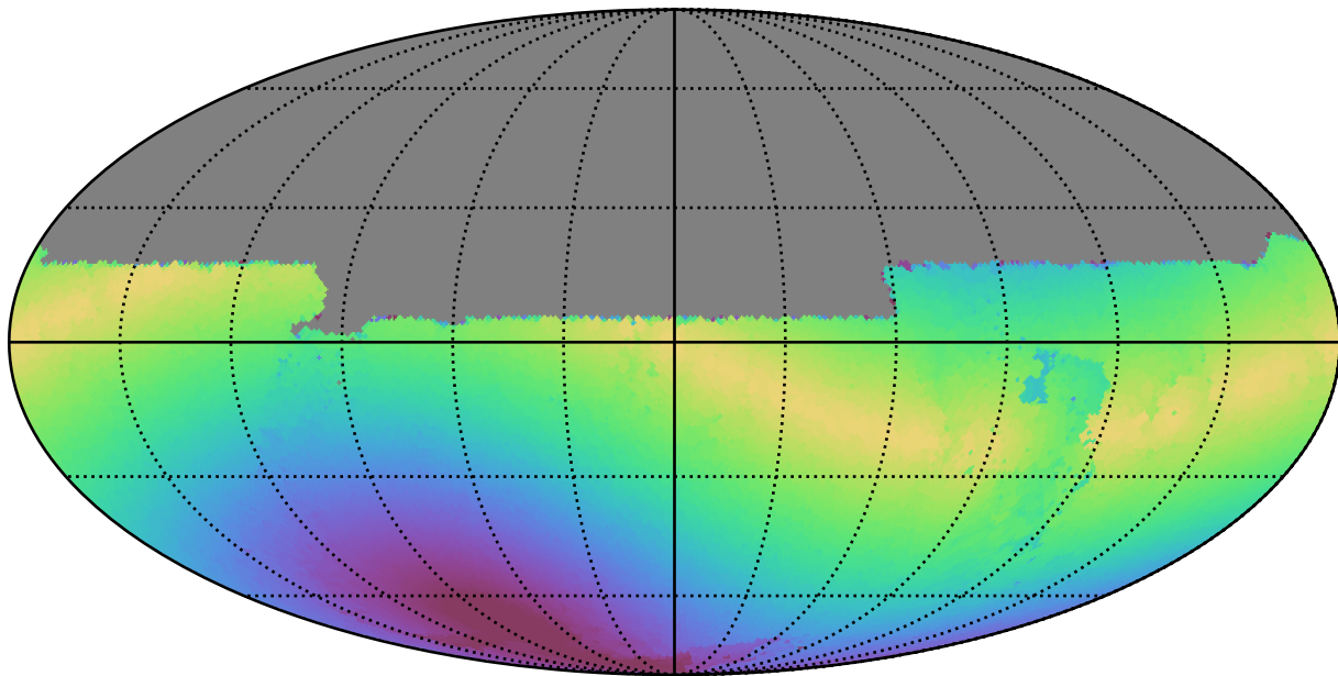
baseline_v3.2_10yrs All sky u band: Max solarElong
