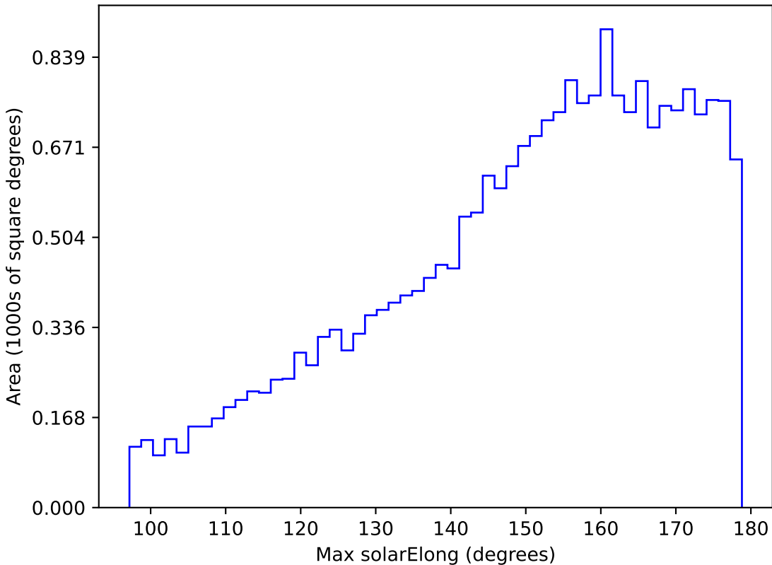
baseline_v3.2_10yrs All sky u band: Max solarElong
