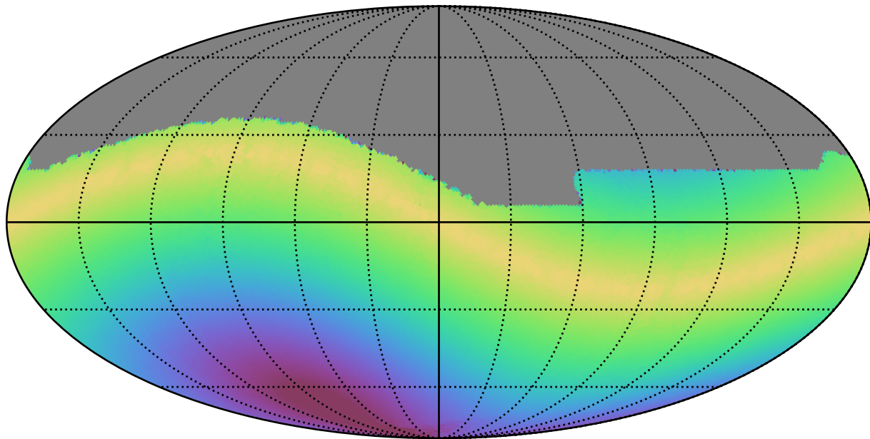
baseline_v3.2_10yrs All sky r band: Max solarElong
