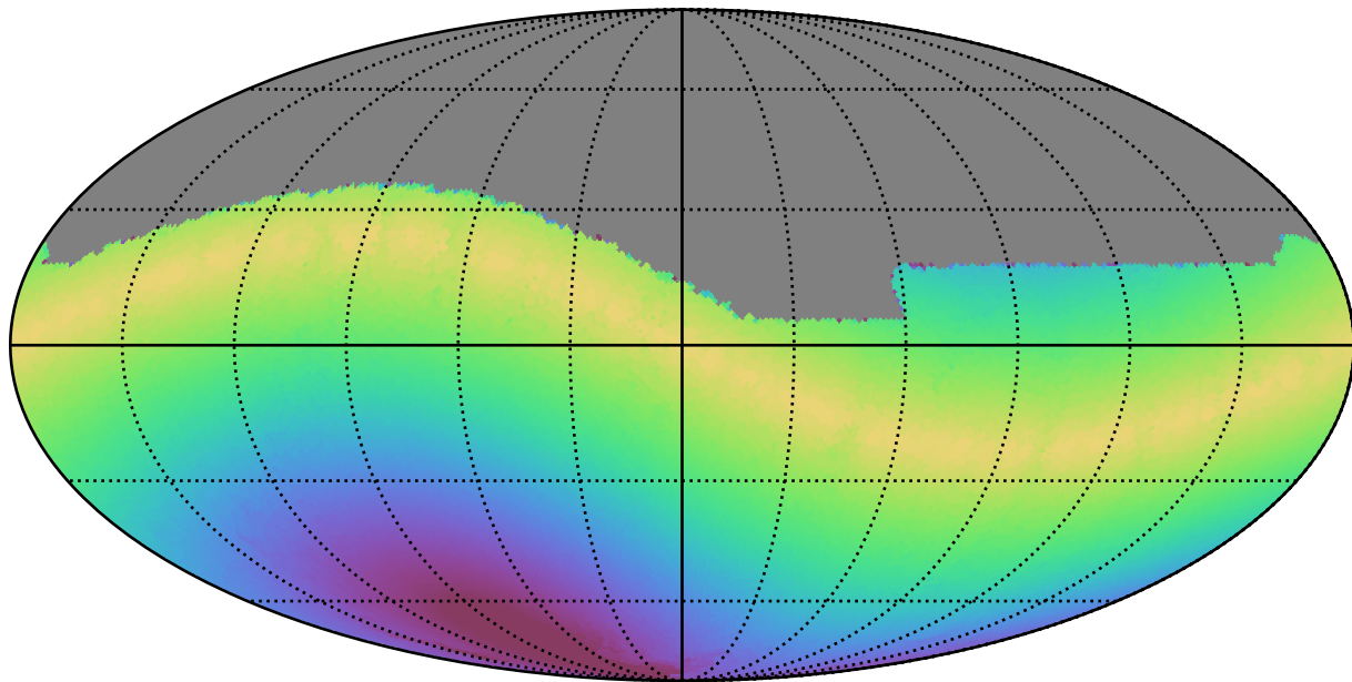
baseline_v3.2_10yrs All sky g band: Max solarElong
