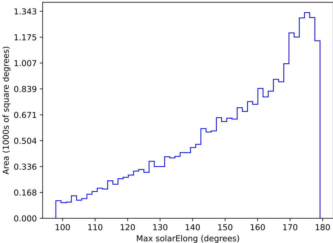
baseline_v3.2_10yrs All sky g band: Max solarElong
