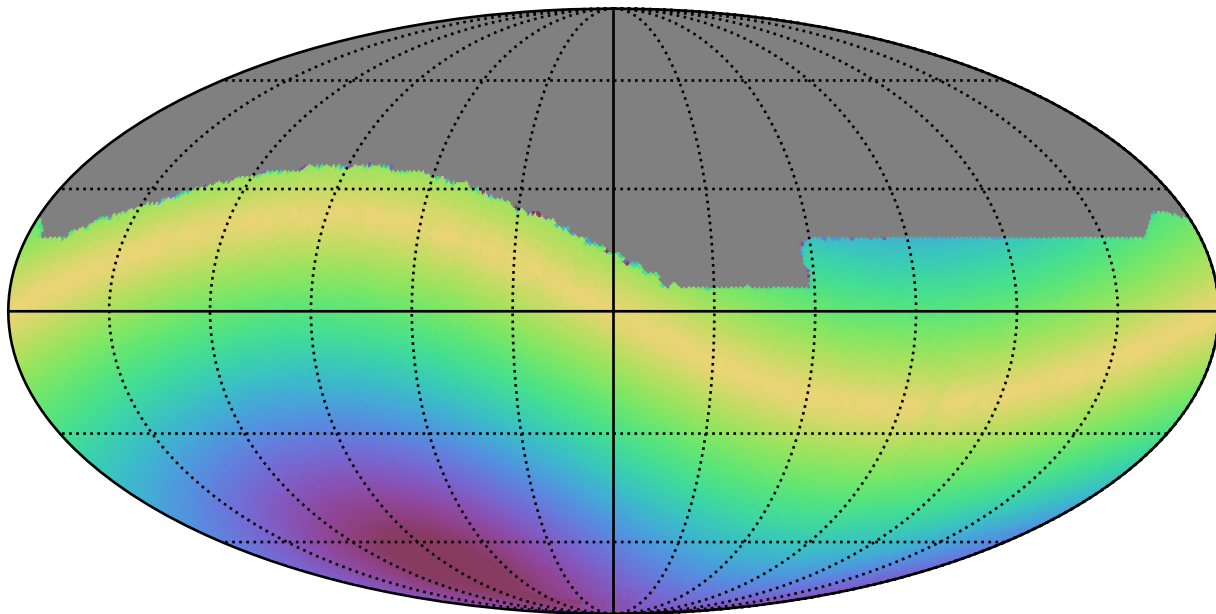
baseline_v3.2_10yrs All sky all bands: Max solarElong
