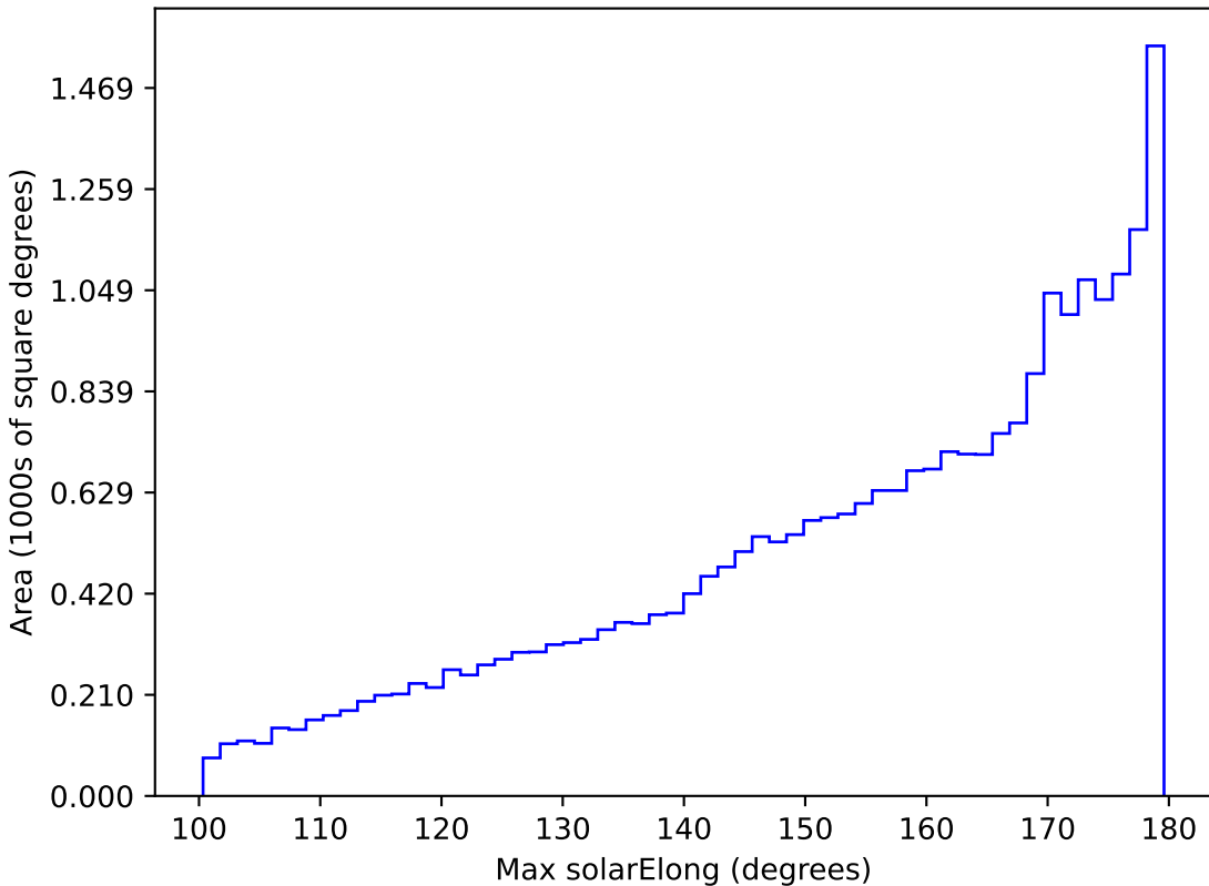
baseline_v3.2_10yrs All sky all bands: Max solarElong
