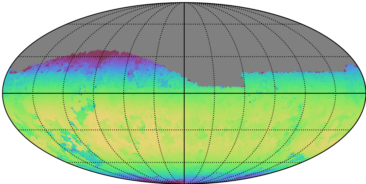
baseline_v3.2_10yrs Yr 1 z band: Max skyBrightness
