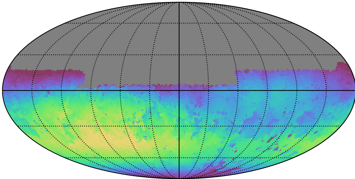
baseline_v3.2_10yrs Yr 1 u band: Max skyBrightness
