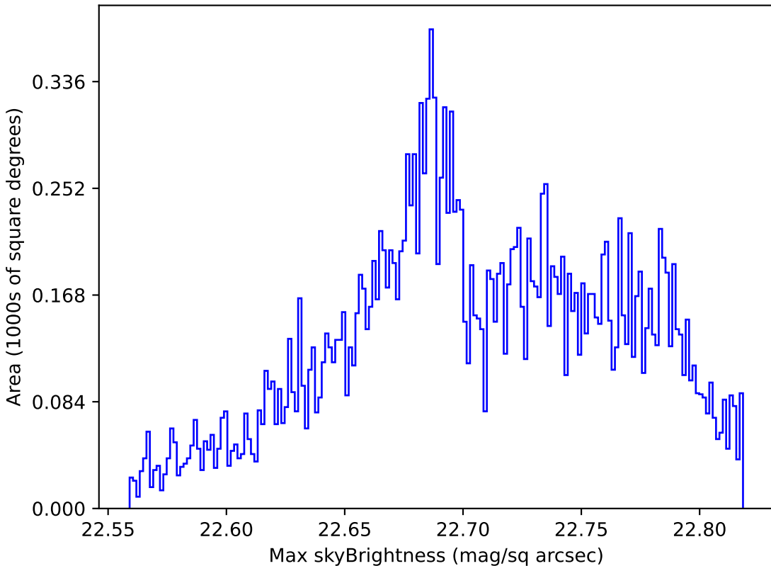
baseline_v3.2_10yrs Yr 1 u band: Max skyBrightness
