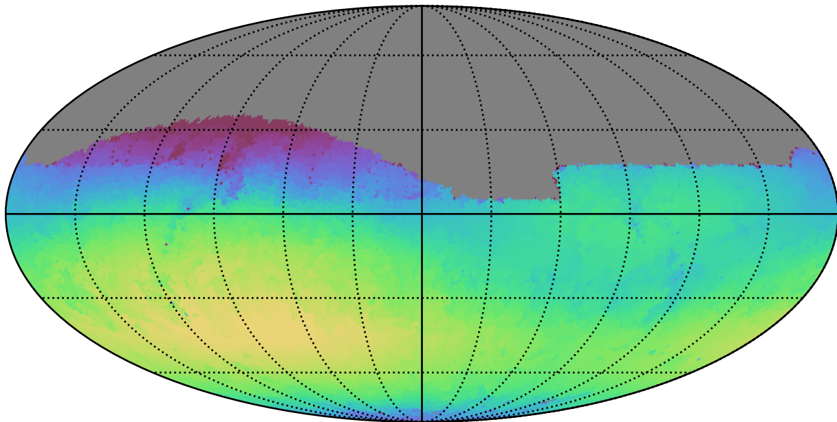
baseline_v3.2_10yrs Yr 1 r band: Max skyBrightness
