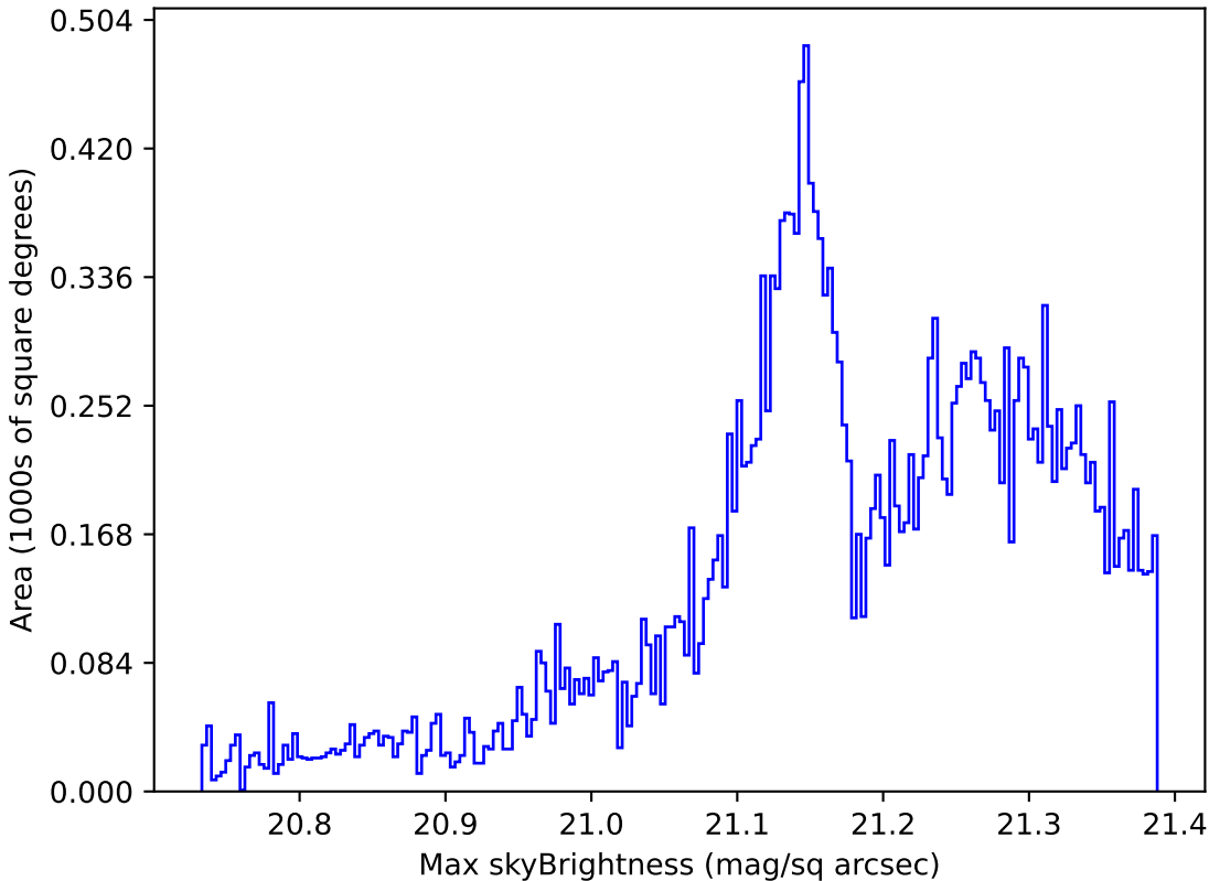
baseline_v3.2_10yrs Yr 1 r band: Max skyBrightness
