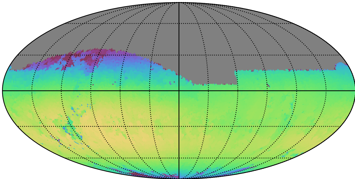
baseline_v3.2_10yrs Yr 1 i band: Max skyBrightness
