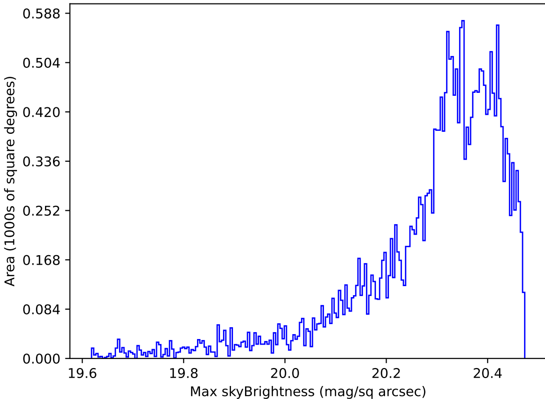
baseline_v3.2_10yrs Yr 1 i band: Max skyBrightness
