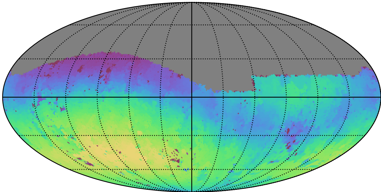
baseline_v3.2_10yrs Yr 1 g band: Max skyBrightness
