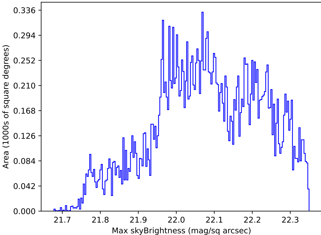
baseline_v3.2_10yrs Yr 1 g band: Max skyBrightness
