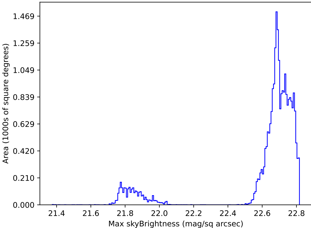
baseline_v3.2_10yrs Yr 1 all bands: Max skyBrightness
