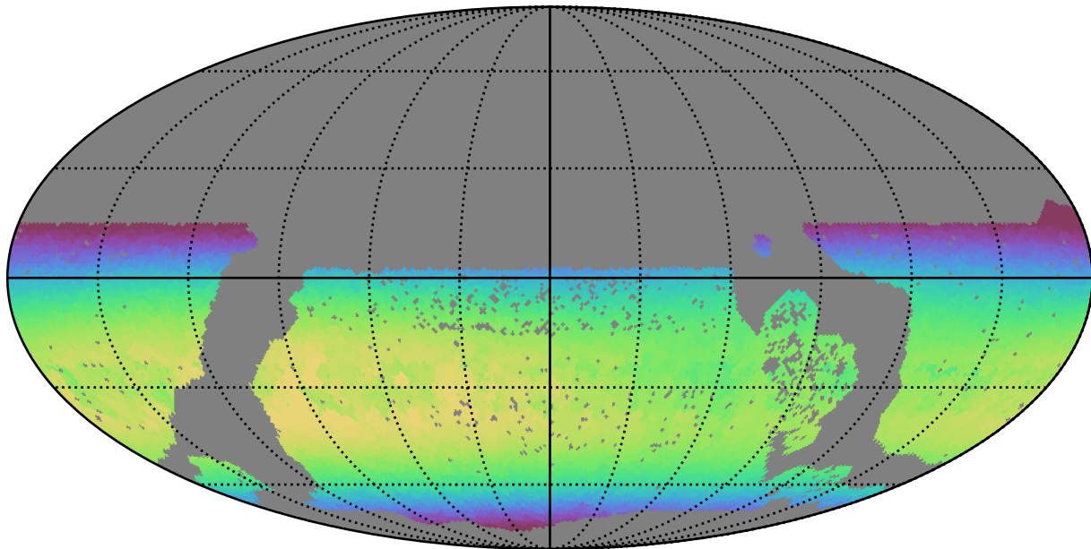
baseline_v3.2_10yrs WFD z band: Max skyBrightness
