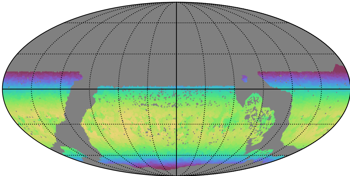
baseline_v3.2_10yrs WFD y band: Max skyBrightness
