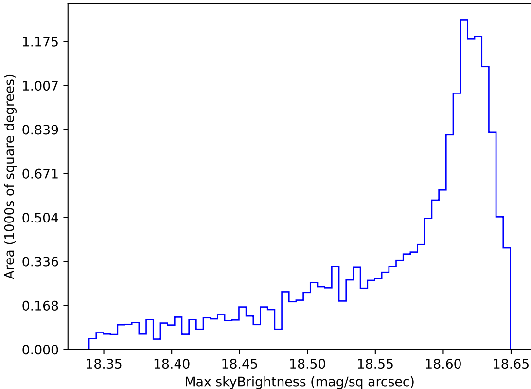
baseline_v3.2_10yrs WFD y band: Max skyBrightness
