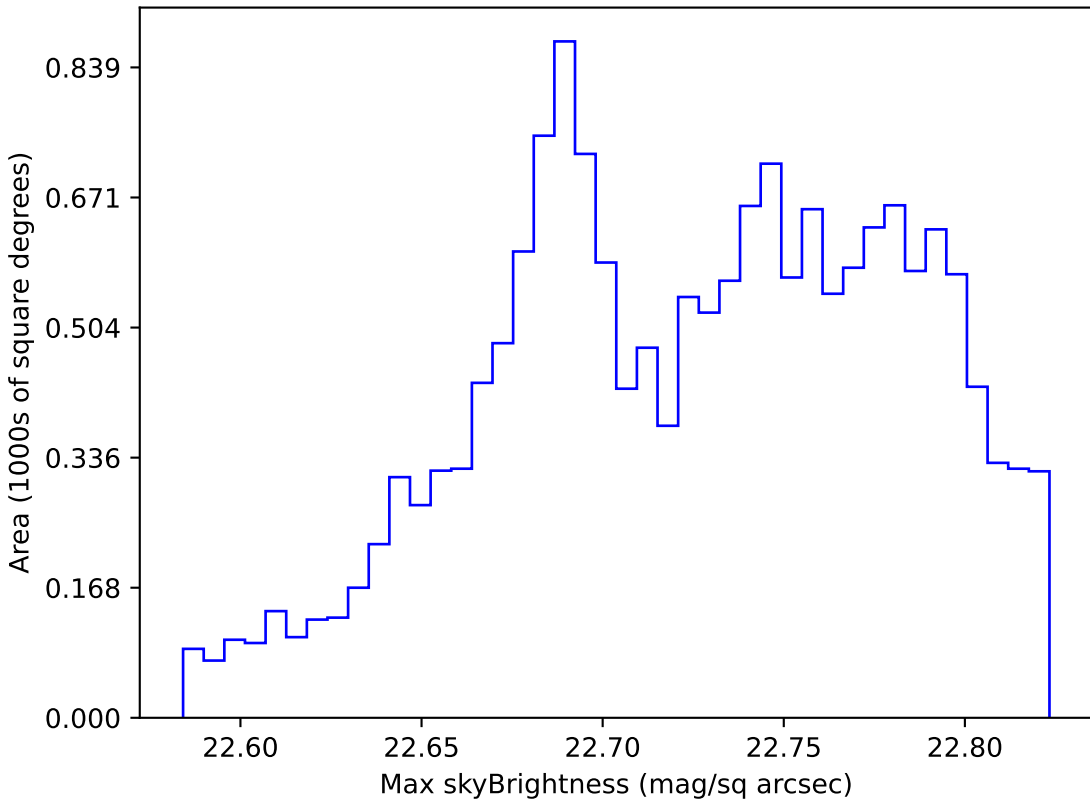
baseline_v3.2_10yrs WFD u band: Max skyBrightness
