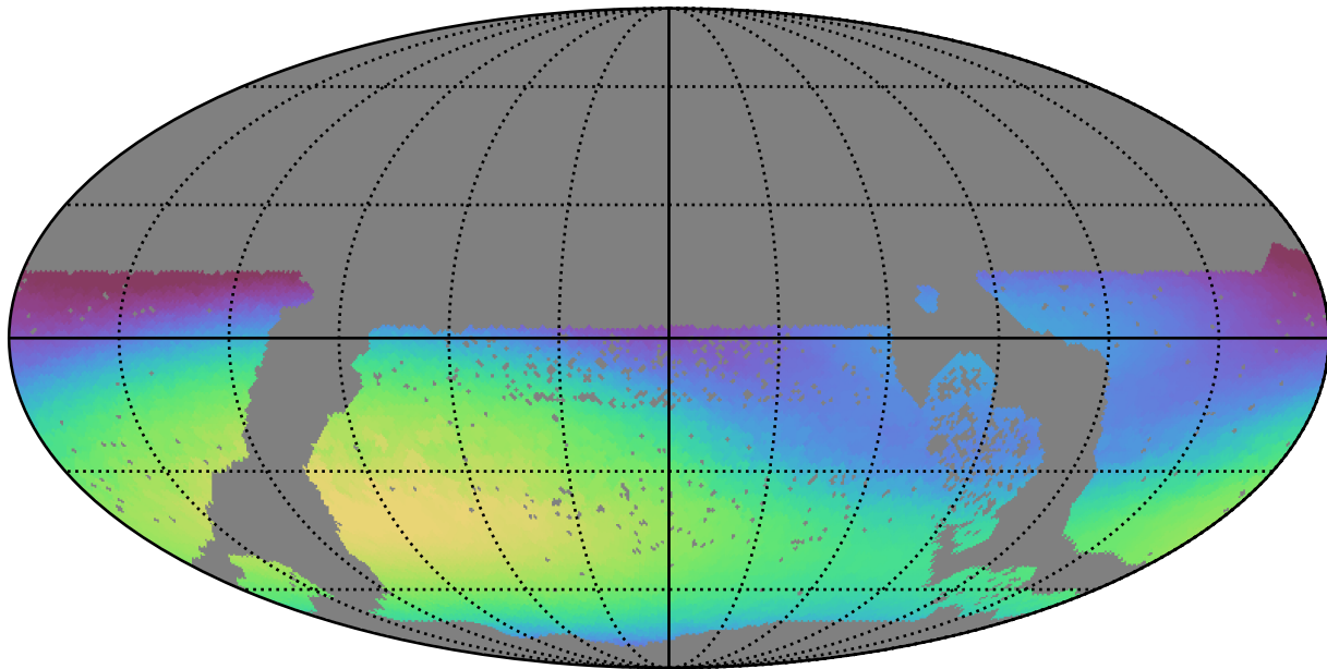
baseline_v3.2_10yrs WFD r band: Max skyBrightness
