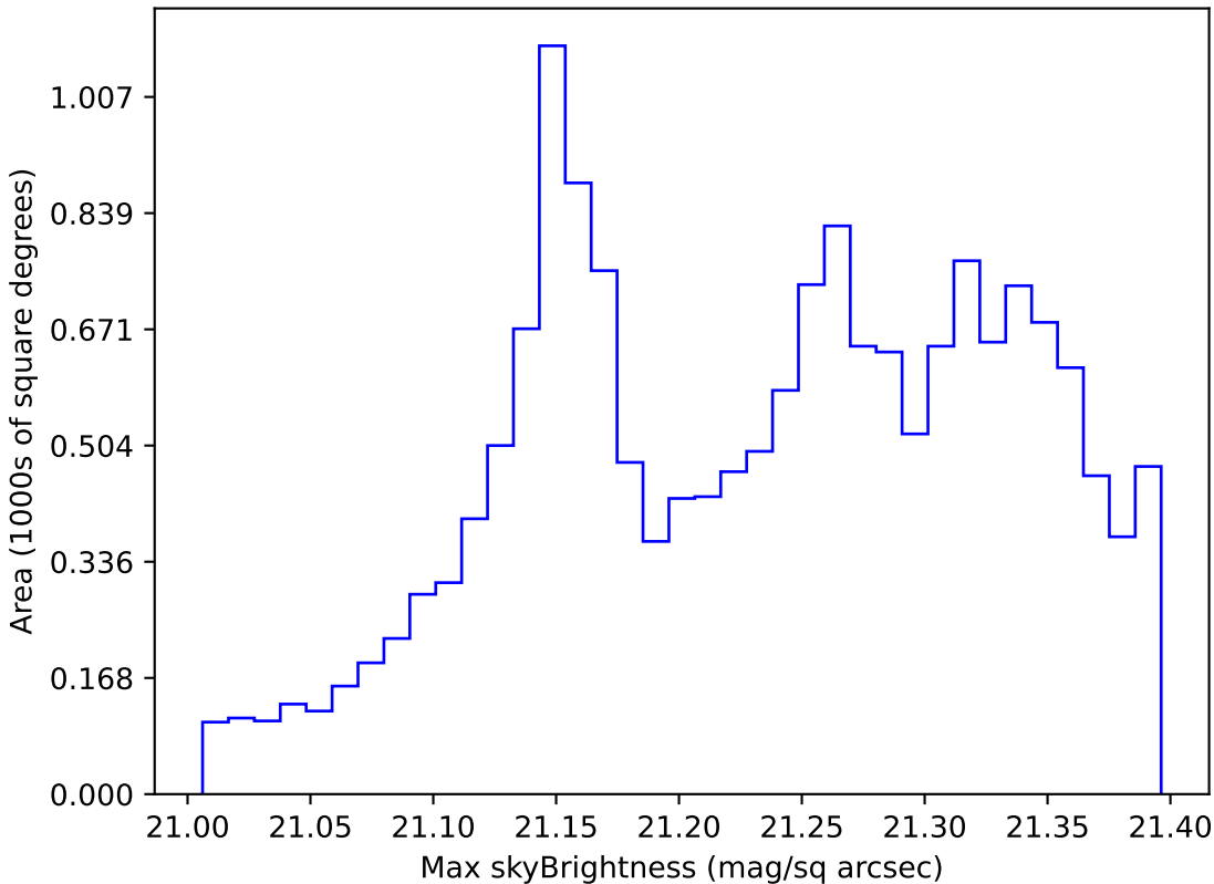
baseline_v3.2_10yrs WFD r band: Max skyBrightness
