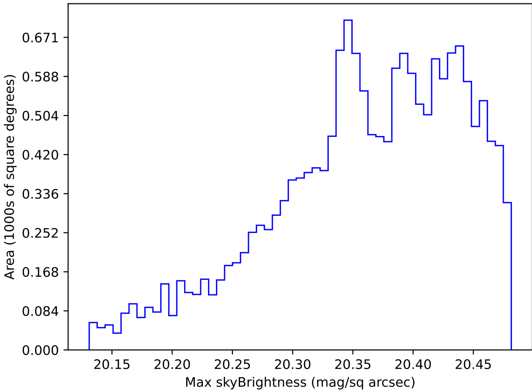
baseline_v3.2_10yrs WFD i band: Max skyBrightness
