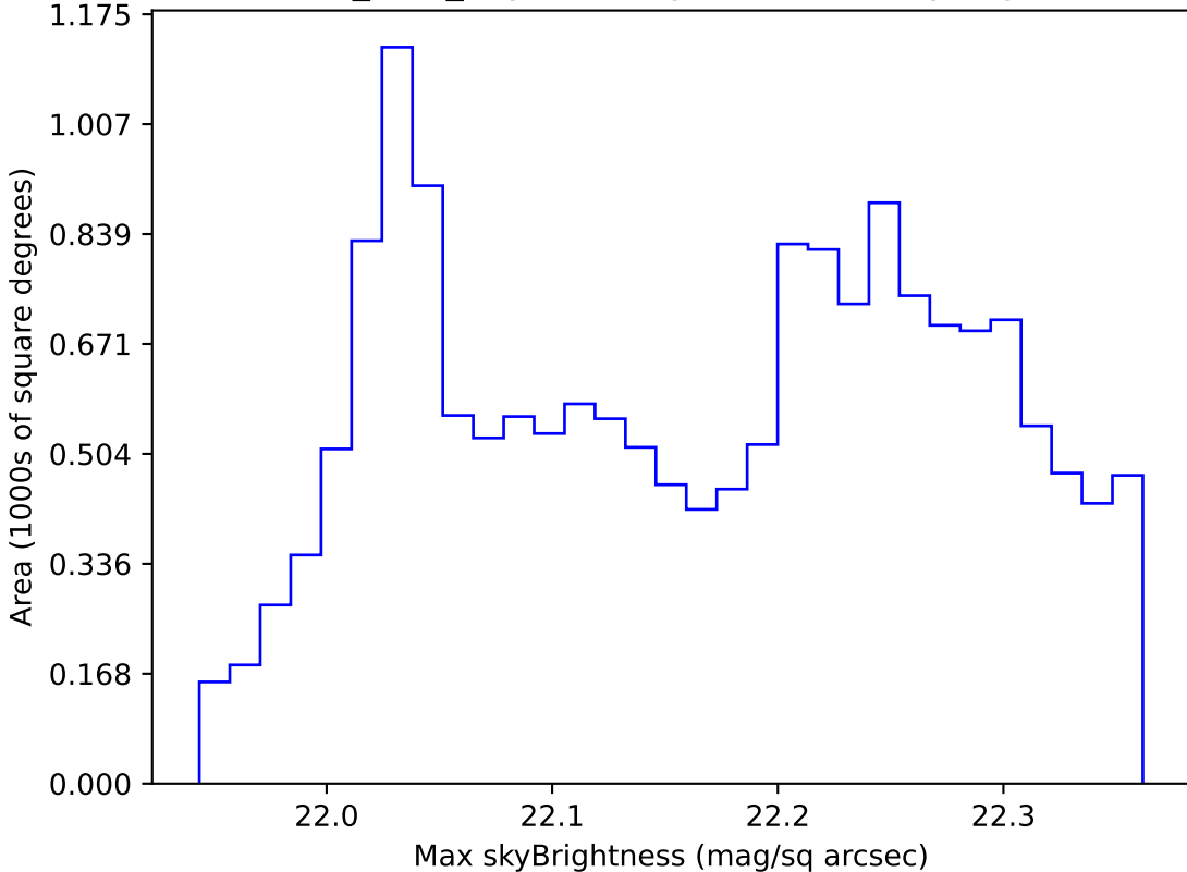
baseline_v3.2_10yrs WFD g band: Max skyBrightness
