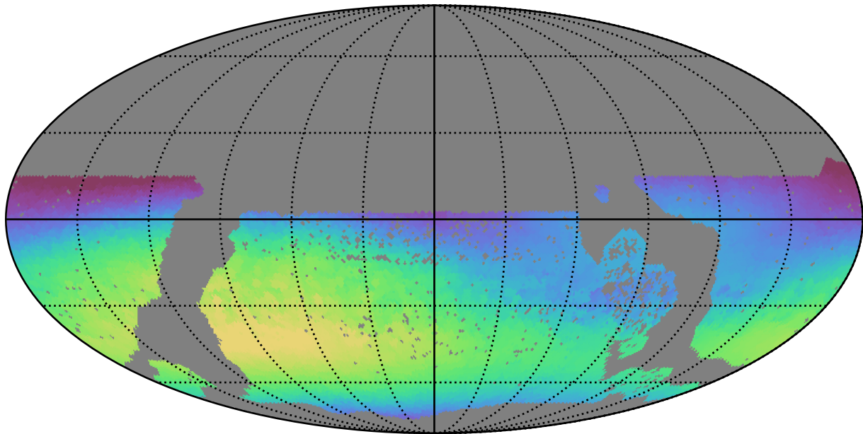
baseline_v3.2_10yrs WFD all bands: Max skyBrightness
