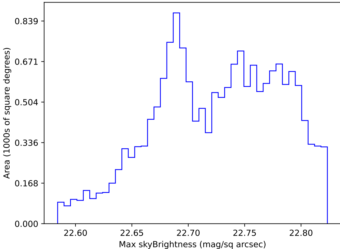
baseline_v3.2_10yrs WFD all bands: Max skyBrightness
