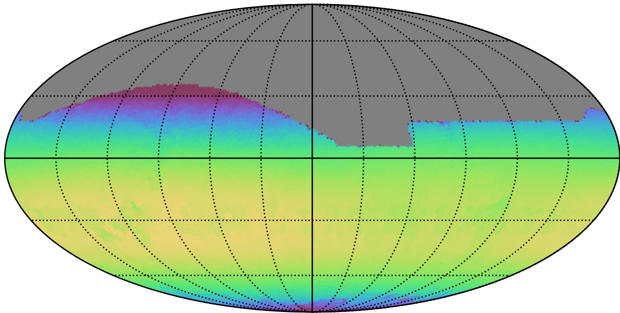
baseline_v3.2_10yrs All sky z band: Max skyBrightness
