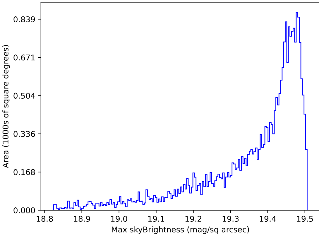
baseline_v3.2_10yrs All sky z band: Max skyBrightness
