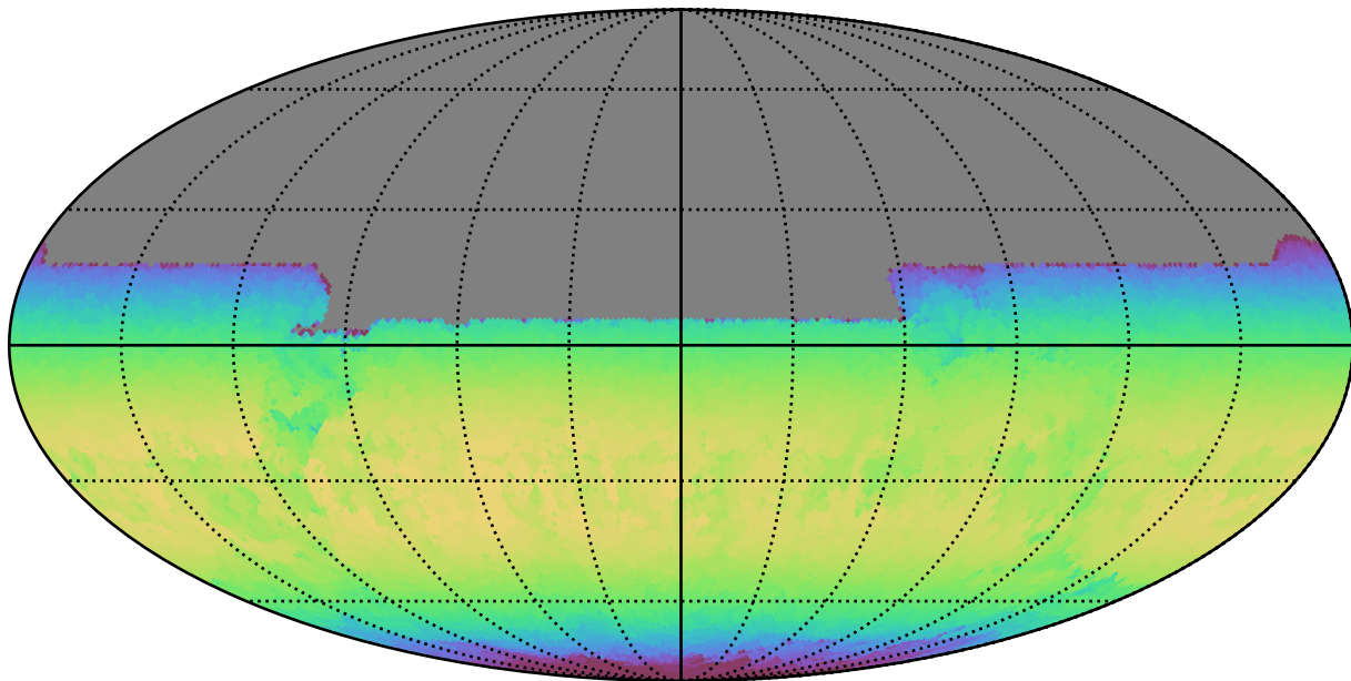
baseline_v3.2_10yrs All sky y band: Max skyBrightness
