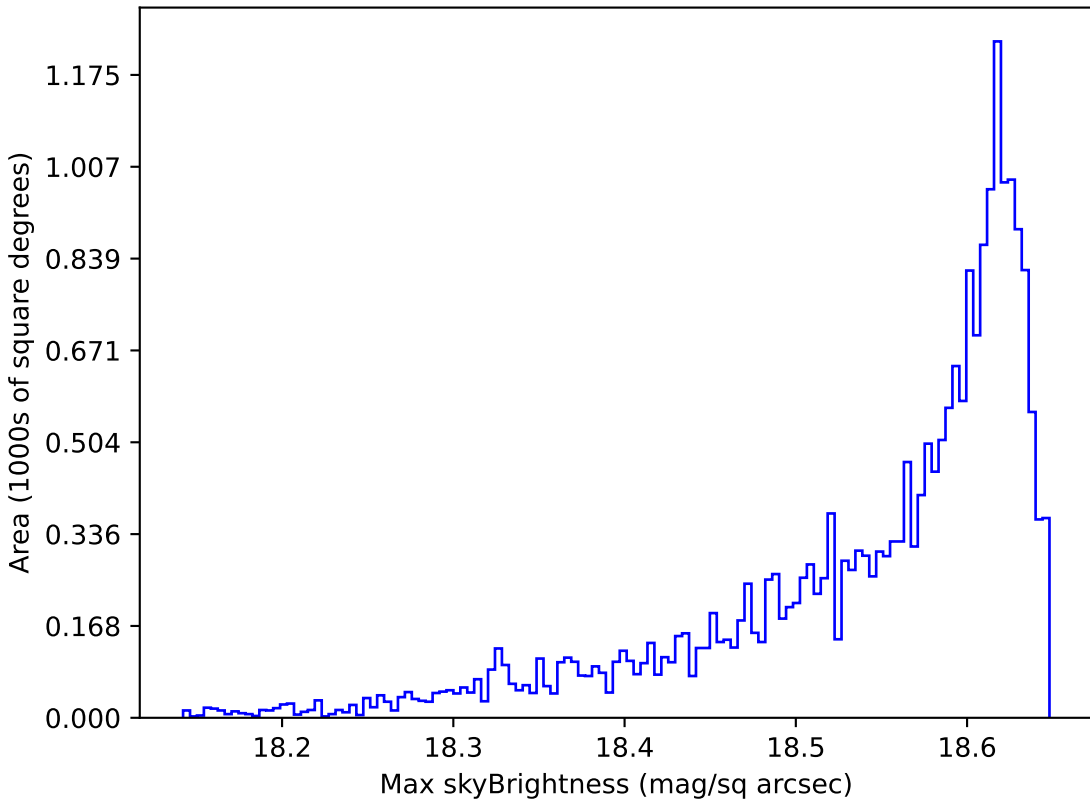
baseline_v3.2_10yrs All sky y band: Max skyBrightness
