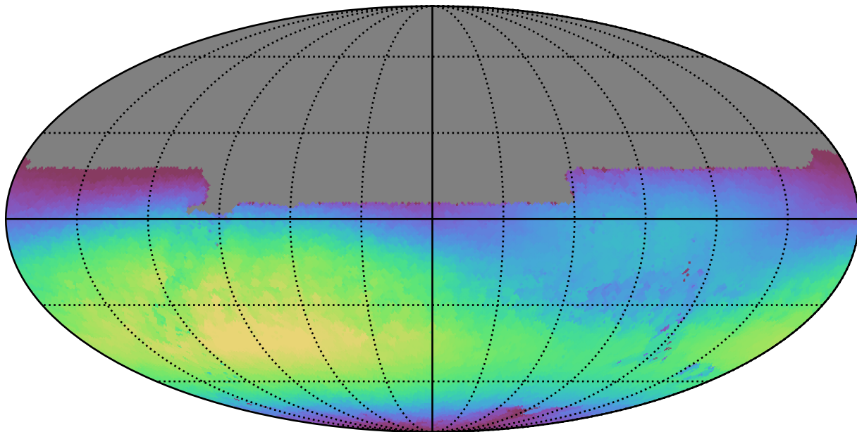
baseline_v3.2_10yrs All sky u band: Max skyBrightness
