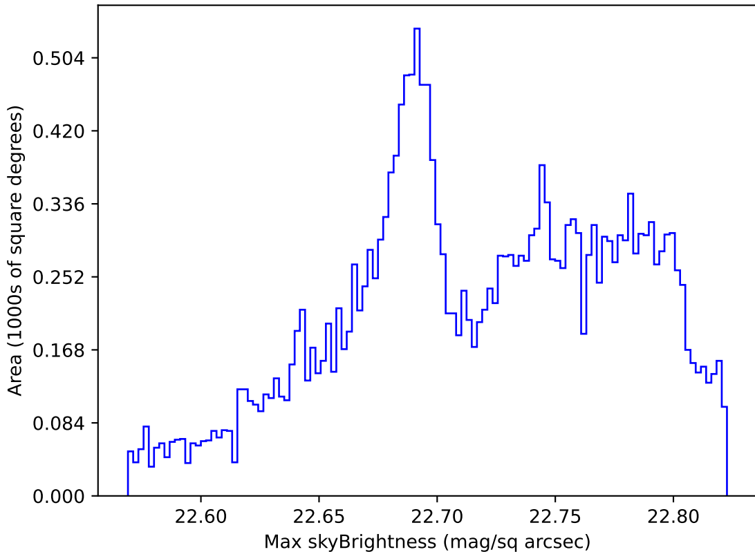
baseline_v3.2_10yrs All sky u band: Max skyBrightness
