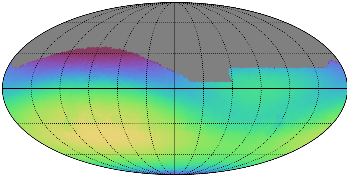
baseline_v3.2_10yrs All sky r band: Max skyBrightness
